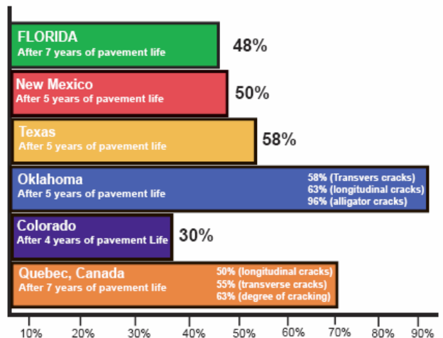
Reduction In Overlay Reflective Cracking With The Petromat System Compared To Control Sections With No Fabric
